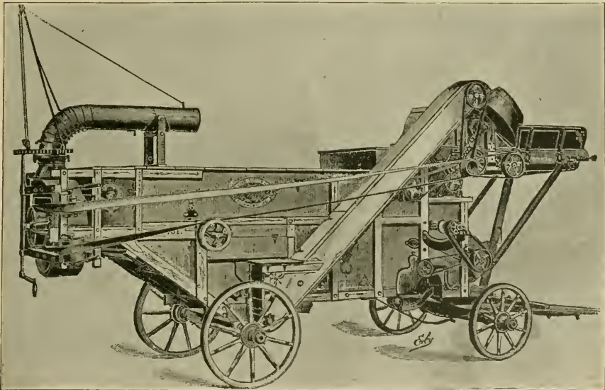
MODERN CLOVER HULLER. Showing Uncle Tom's Stacker and Self-Feeder.
